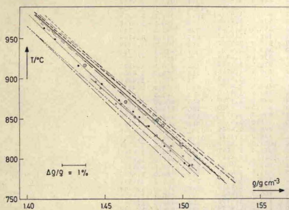
Fig. 5. Density of molten potassium chloride as a function of temperature at 1 bar. — Grjotheim et al. (1971) 15 , — Kirshenbaum et al. (1962) 16 , ●····· Neithamer and Peake (1961) 17 , — Van Artsdalen and Yaffe (1955) 18 , ○ Peake and Bothwell (1954) 20 , —····· Bloom et al. (1953) 21 , —····· Mashovetz and Lundina (1935) 22 , —····· Klemm (1926) 23 , —····· Jäger (1917) 25 , —····· Brunner (1904) 26 , ⊙ This work.
